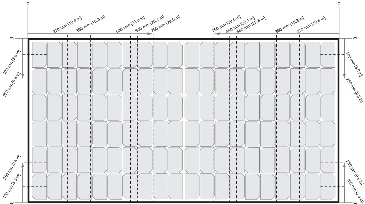
Fig. 8: Clamping of REC TwinPeak 5 Series panels using short rails
